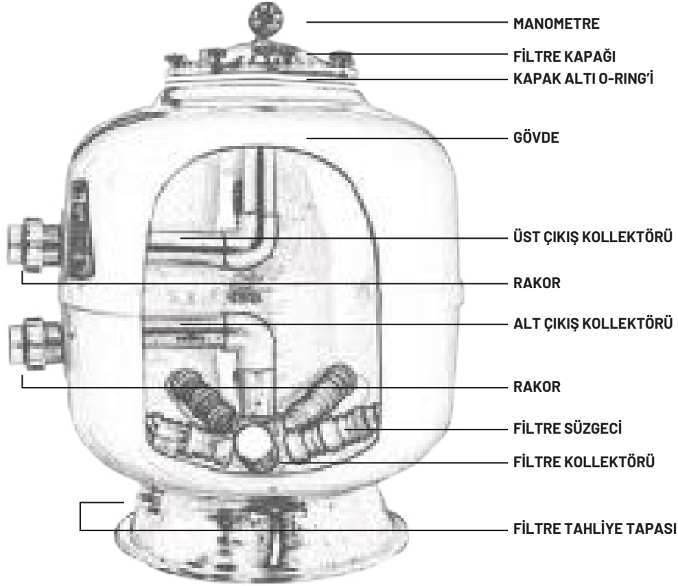
Atlaspool Pool Filters Spare Parts List
