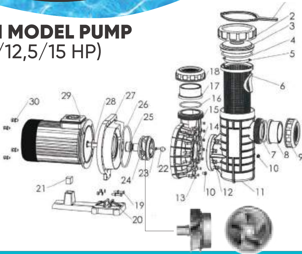
Atlaspool Pool Pumps Spare Parts List
