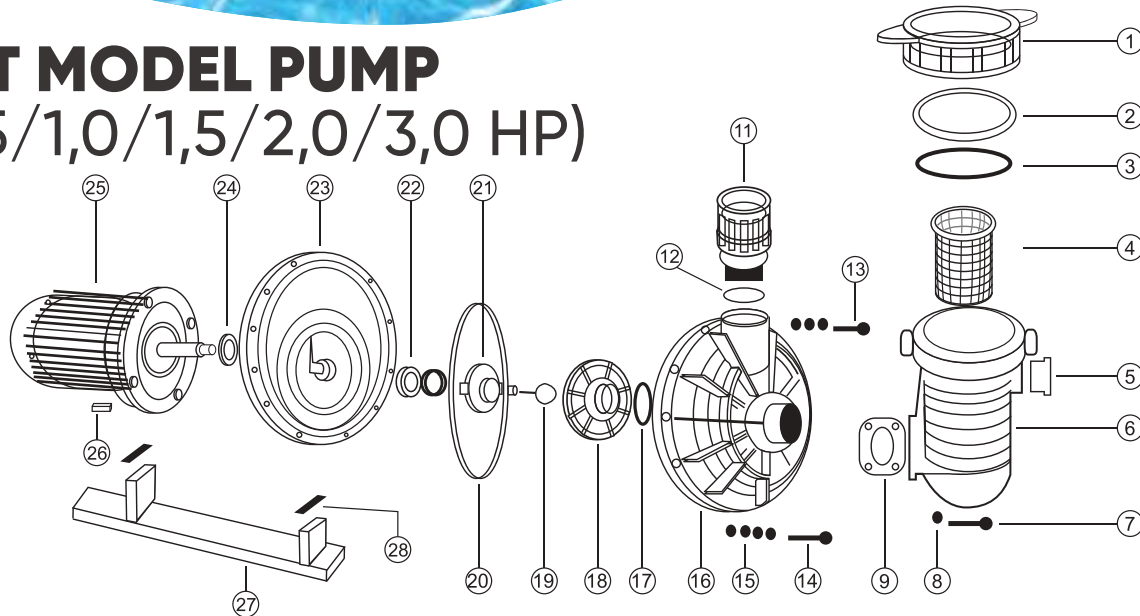
Atlaspool Pool Pumps Spare Part List
