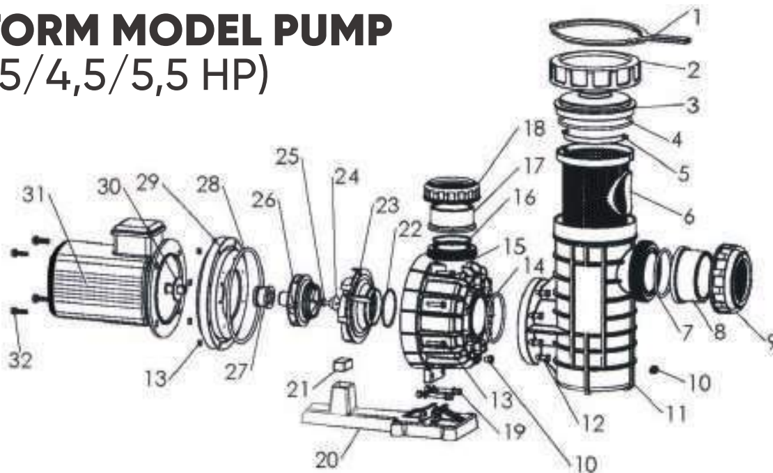
Atlaspool Pool Pumps Spare Parts List
